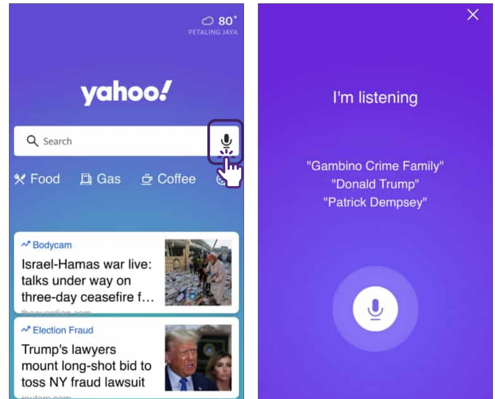
Yahoo Search
