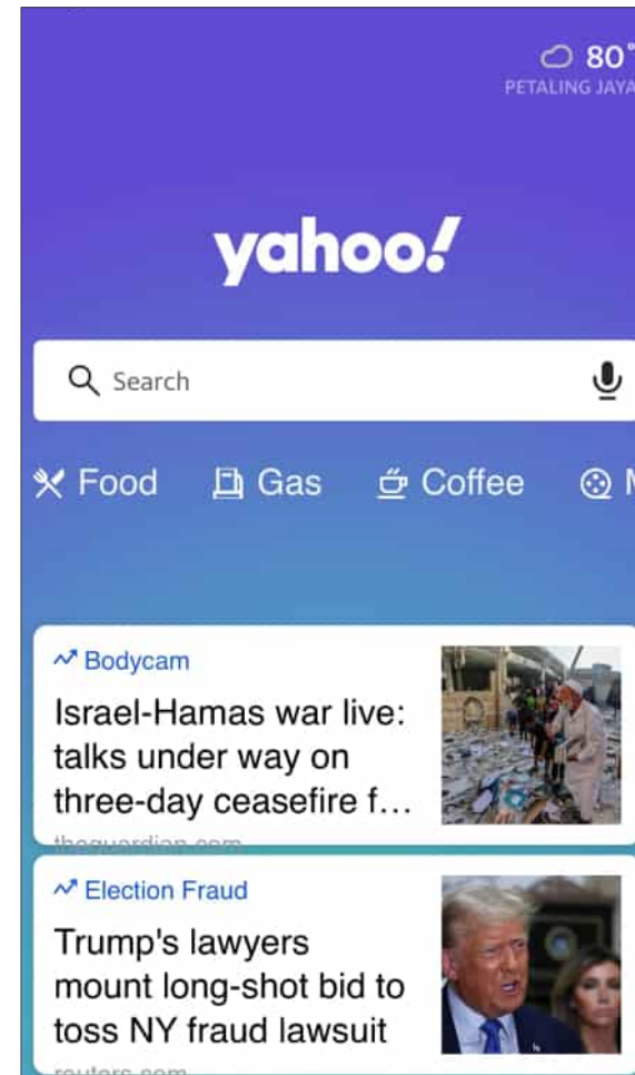
Yahoo Search
