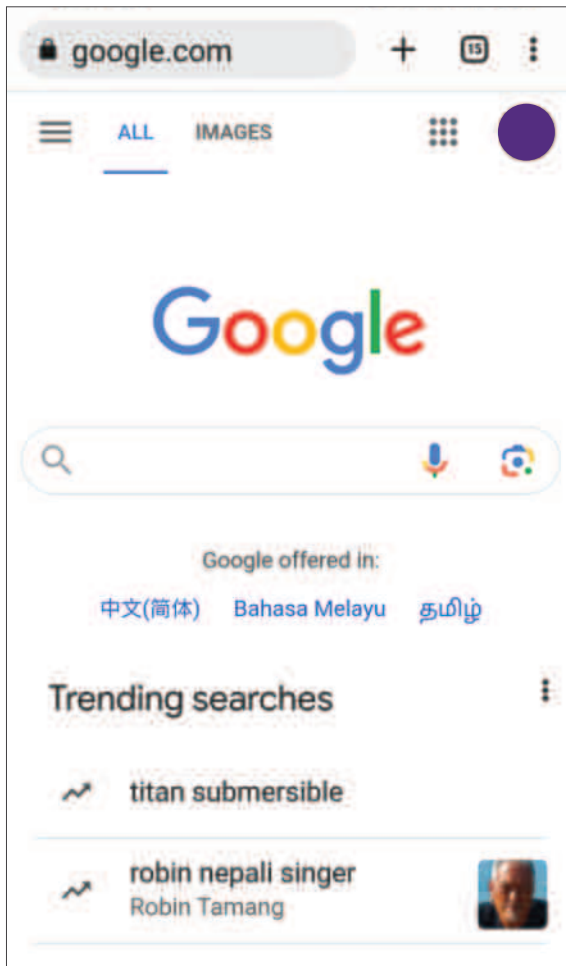
Google Search
